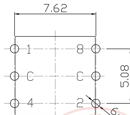
P.C.B. DIMENSION (TOP VIEW)
