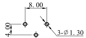
PCB LAYOUT
