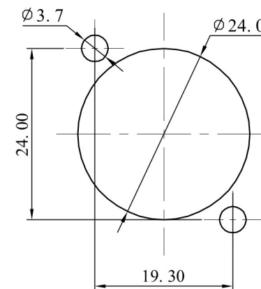
PANEL CUTOUT
